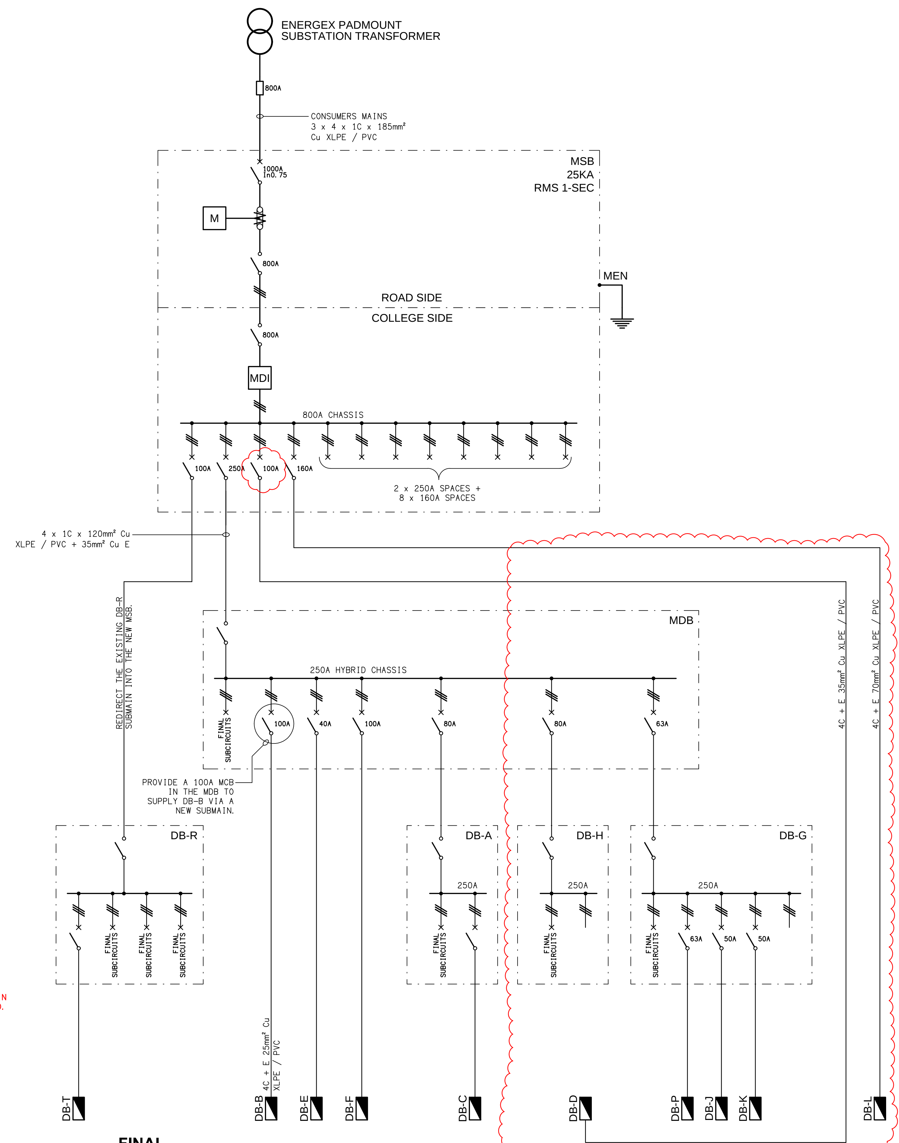
FINAL POWER DISTRIBUTION SCHEMATIC NOT TO SCALE
