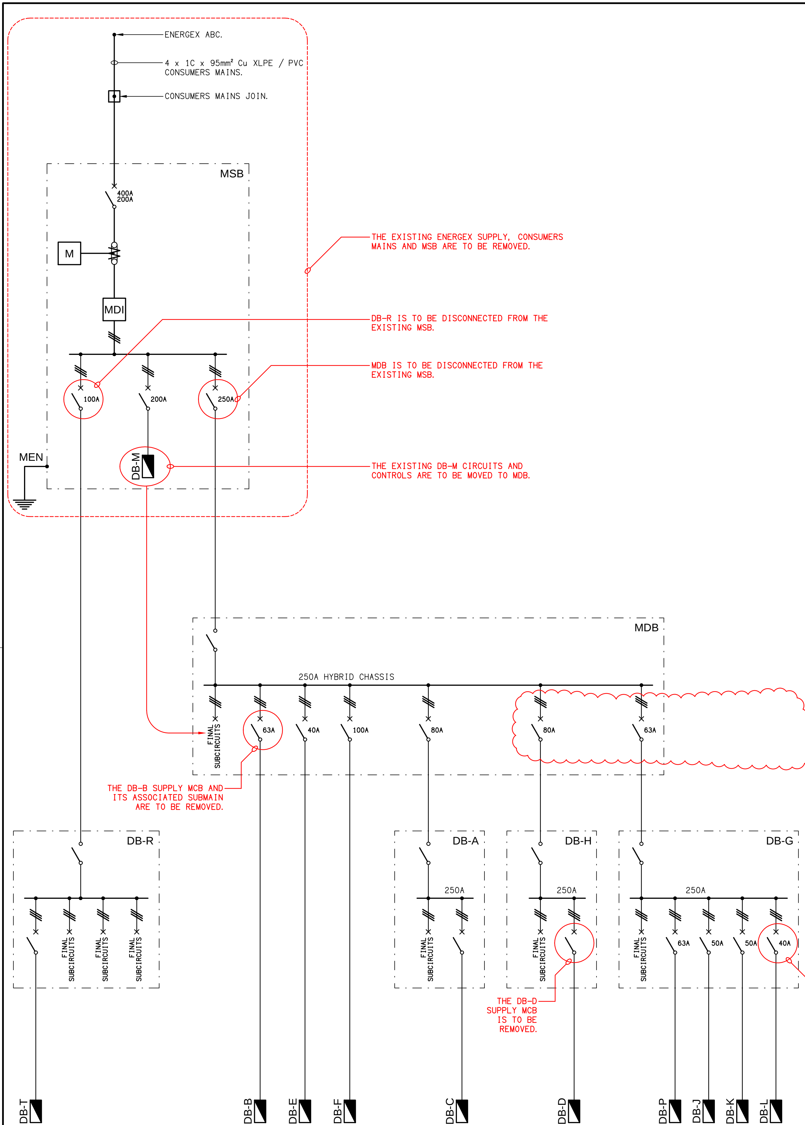
EXISTING MODIFIED POWER DISTRIBUTION SCHEMATIC NOT TO SCALE
